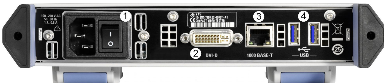
Fig. 4-2: Rear panel view
